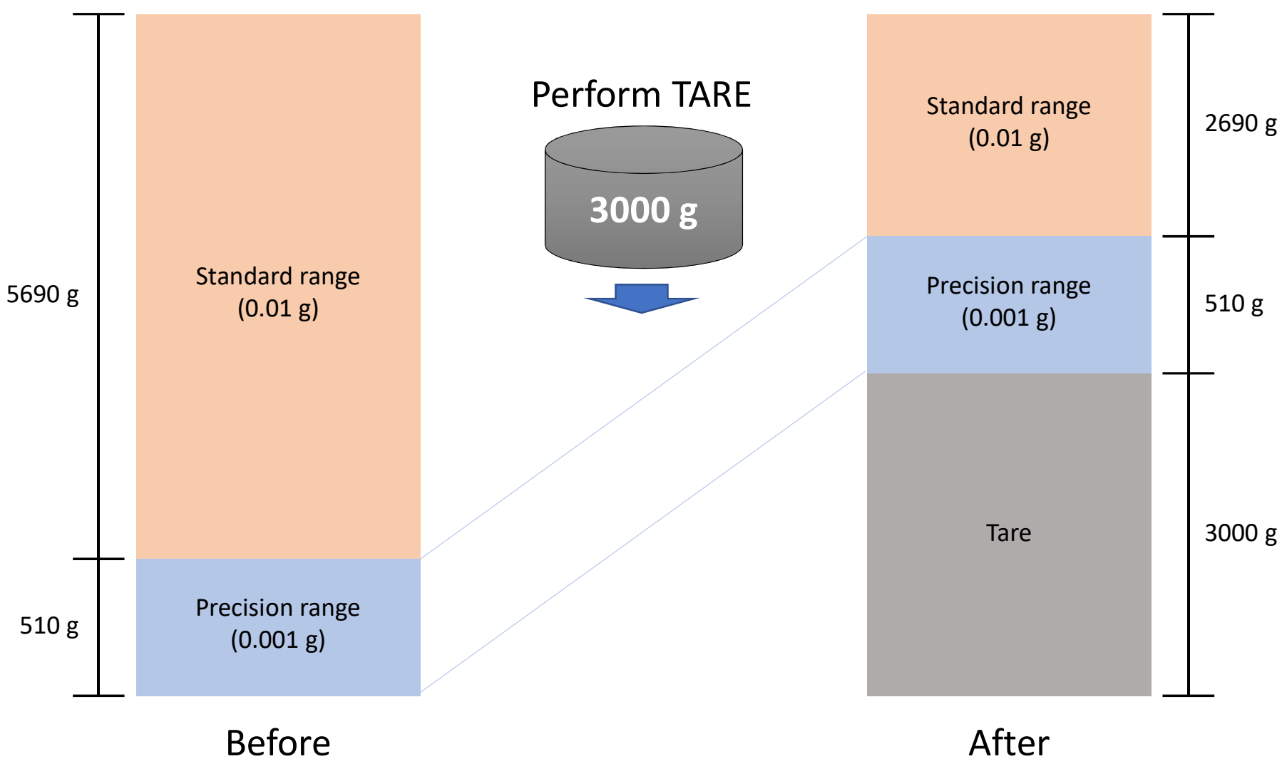
Precision range (0.001 g) of the AD-4212F-6203D before/after performing tare
