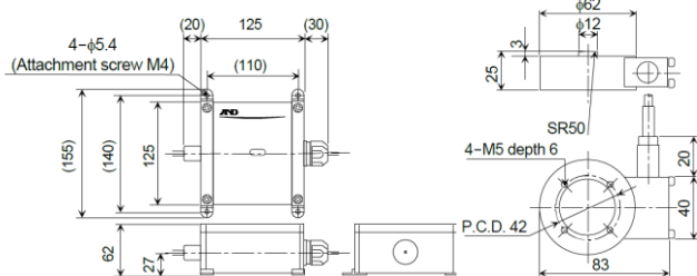
External View CONVERSION BOX
